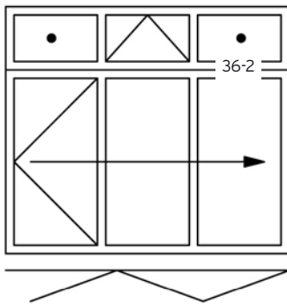
Folding façade with turn and tilt panel in the folding façade
