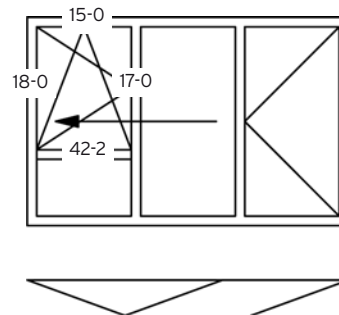
Folding façade with turn and tilt panel
