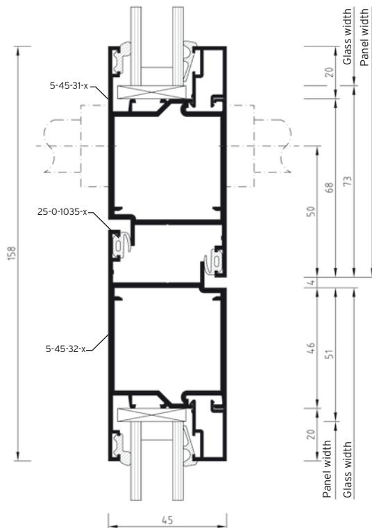
Detail 45-72-4
