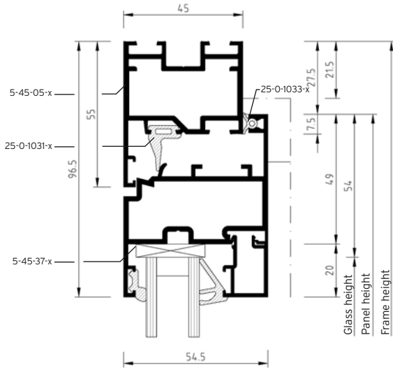
Detail 45-40-0
