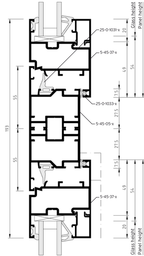
Detail 45-44-0
