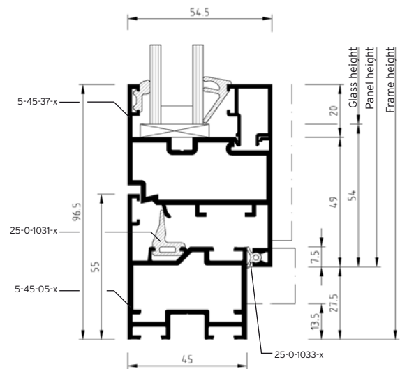
Detail 45-40-2
