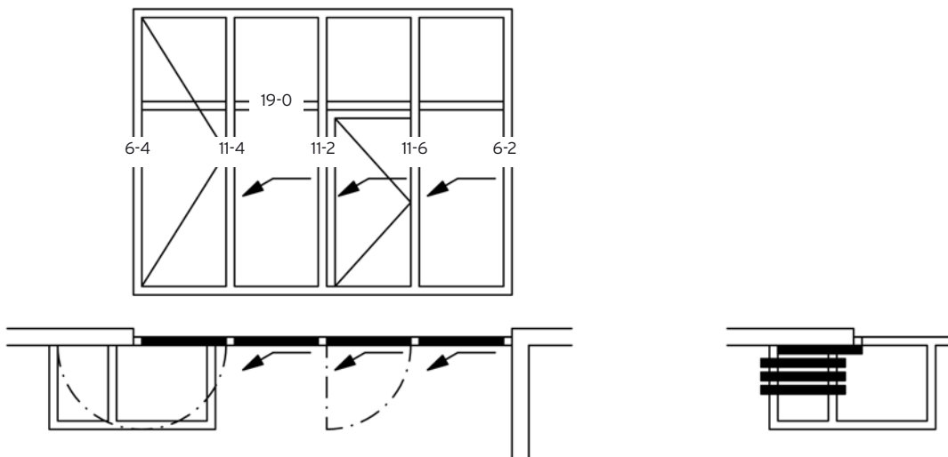
HSW with panel with incorporated pass door and transom rail
