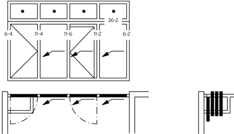
HSW with panel with incorporated pass door and transom window
