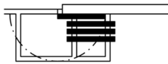
Stacking bay outside the plane of the opening on top of 180° turned swing panel
