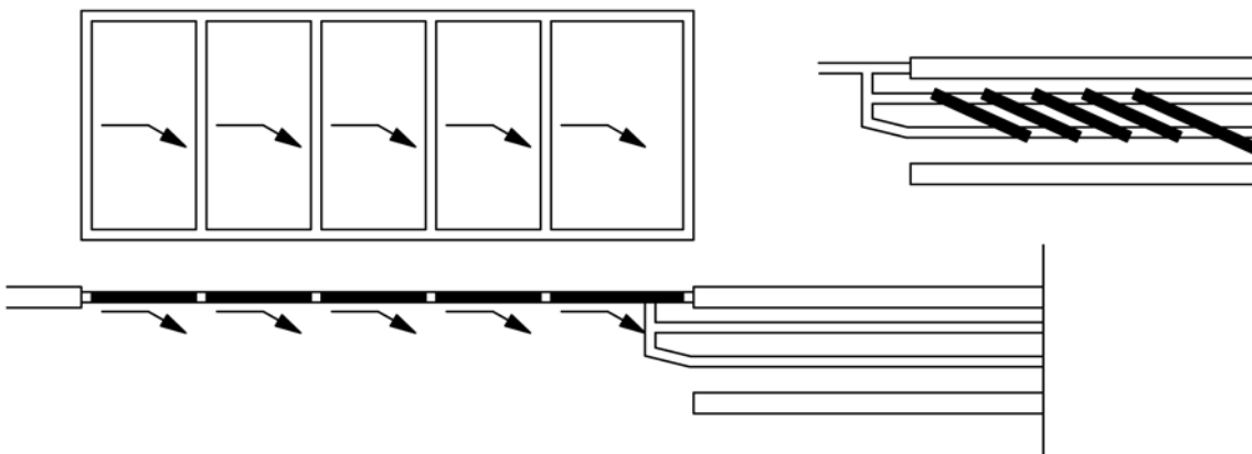
Straight configuration with stacking inside pocket
