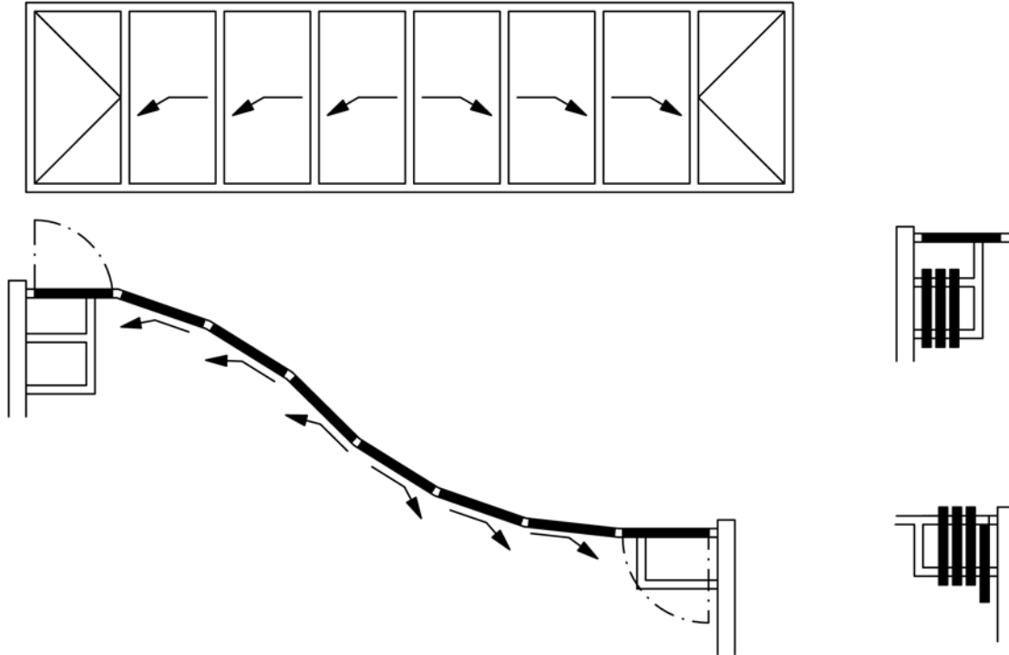
S-shaped configuration (plan view)
