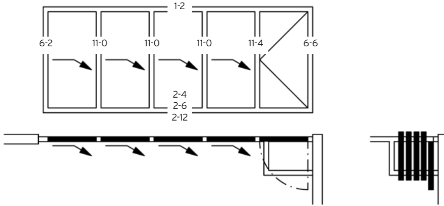
Straight configuration (plan view)
