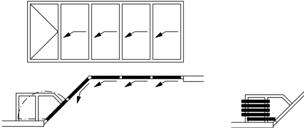
Angled configuration (plan view)
