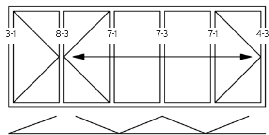
A - 1L 4LR Swing
